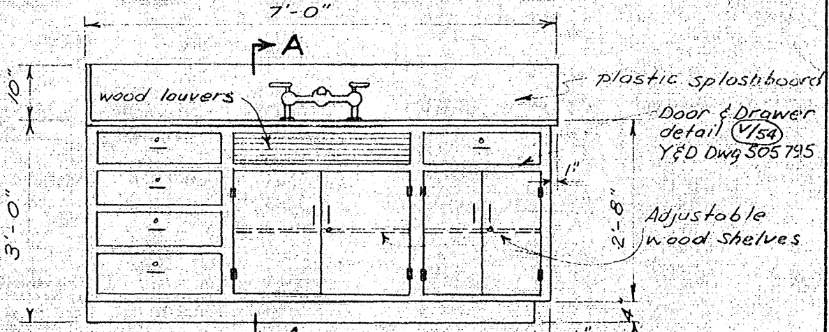
ELEVATION Scale 1/2" = 1'-0"
