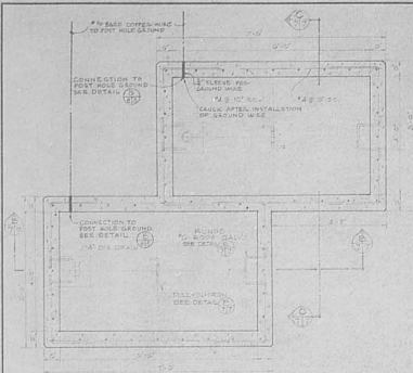
PLAN SCALE 1/4" = 1'-0"
