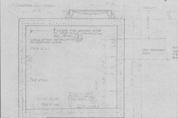
PLAN SCALE 1/4" = 1'-0"
