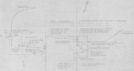
ELECTRICAL SERVICE EQUIPMENT LAYOUT & POWER WIRING PLAN SCALE 1/4" = 1'-0"
